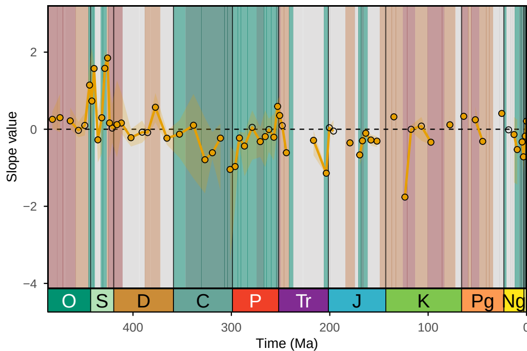
B Southern Hemisphere
